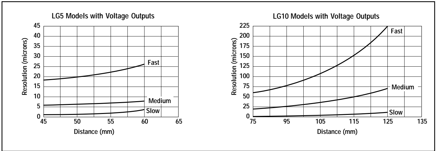
Figure 3. L-GAGE resolution, with respect to speed (typical, using a white ceramic target)
