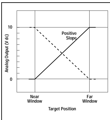
Figure 6. Analog output as a function of target position
