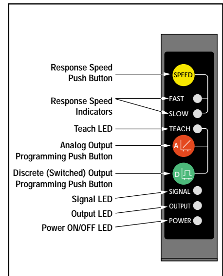
Figure 4. L-GAGE™ Laser Gauging Sensor programming push buttons and indicators
