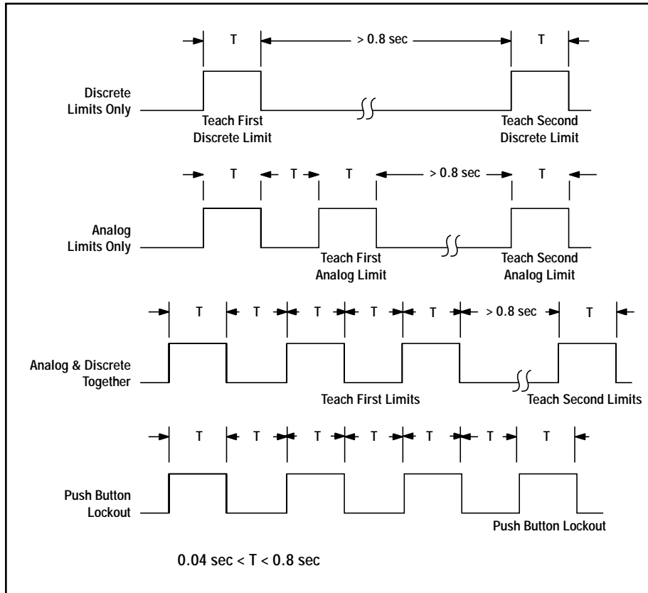
Figure 5. Timing programs for remote TEACH programming
