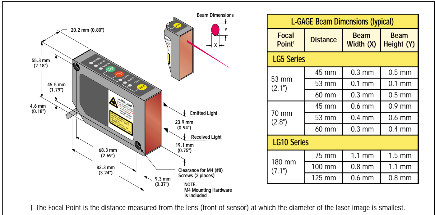
Figure 2. L-GAGE Laser Gauging Sensor and beam dimensions
