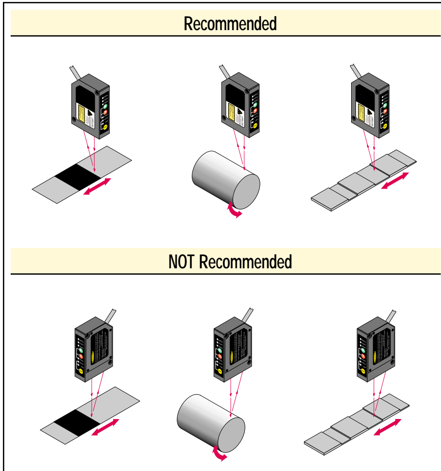
Figure 7. Sensor orientations for typical targets
